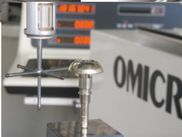
Controllo Control
